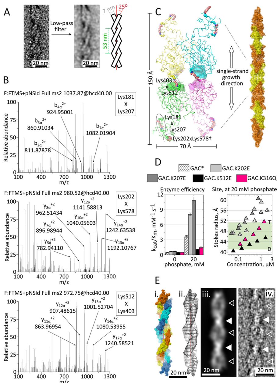
FIGURE 4. A model of GAC superoligomer assembly. A , the removal of high frequencies (strongly associated with noise) from the TEM micrographs highlights the right-handed double-strand nature of the superoligomer, allowing the determination of its geometric features. B , cross-linked MS/MS spectra were manually validated for b and y ion series of the \alpha and \beta chains of cross-linked peptides (between residues Lys 181 and Lys 207 , Lys 202 and Lys 578 , and Lys 403 and Lys 512 ). The ions are indicated by arrows with corresponding m/z value. C , relative position of DSS-linked lysine pairs in the tetramer, as identified by MS. The boundaries of the active sites are delimited by solid surfaces. †, Lys 578 is not modeled in the crystal structure. The proposed single strand growth direction is across the longest axis of the tetramer, via an end to end interaction between pairs of N-terminal domains. Alternating orange and yellow colors facilitate the identification of the tetramers along the single strand. D , one lysine residue from each cross-linked pair was individually substituted by a glutamate and assayed for enzymatic activity ( left panel ) and superstructure formation ( right panel ). The N-terminal region mutants (GAC.K207E and GAC.K207E) enhanced both effects. On the other hand, GAC.K512E, within the glutaminase domain, generated a nonfunctional protein, similarly to the acetylation mimetic GAC.K316Q. The green region delimits the expected Stokes radii between GAC dimers ( D ) and tetramers ( T ), calculated based on the crystal structure dimensions. The asterisk indicates a previously published result for wild-type GAC (5). E , the double strand was manually modeled ( panel i ), using two entwined copies of the single strand from C and following the geometric restrictions of A . In panel ii , the calculated Fourier F_{calc} map (with amplitudes and phases from the double strand model)—limited to 35 Å maximum resolution—is two-dimensionally projected, and the end result is shown in panel iii . All features are comparable to those observed in panel iv , concerning the presence of alternating high density narrow regions (indicated by filled triangles) and low density broad, disc-like regions (indicated by open triangles).
