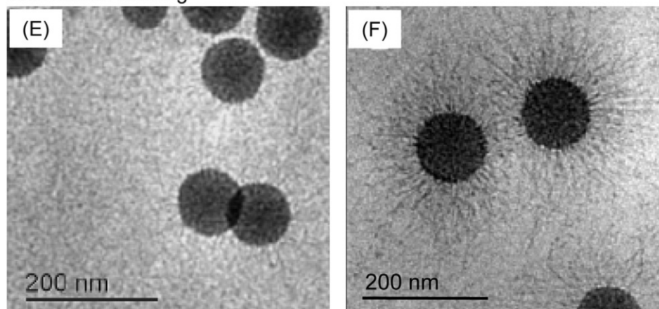
Fig. 9. Cryo-TEM images of a dispersion of poly-2-vinylpyridine 66 -b-poly(ethylene oxide) 46 block co-polymer (P2VP-PEO) micelles after storage at 4 °C and subsequent warming to 16 °C (A–C) and to 25 °C (D). Images were taken after 1 h (A, D), 2.5 h (B) and after 24 h (C). Cryo-TEM images of a 1% suspension of spherical poly(styrene) nanoparticles grafted with long chain poly(styrene sulfonate acid) prepared by photoemulsion polymerization (E and F) at low salt concentration in the medium where the polyelectrolyte chains are strongly stretched. Compared to the original preparation (E) the contrast is enhanced by replacement of the sodium counterions by caesium ions and the addition of bovine serum albumin (F). Reprinted with permission from Rank et al. (2009), American Chemical Society (A–D) and with permission from Wittemann et al. (2005), American Chemical Society (E and F).
