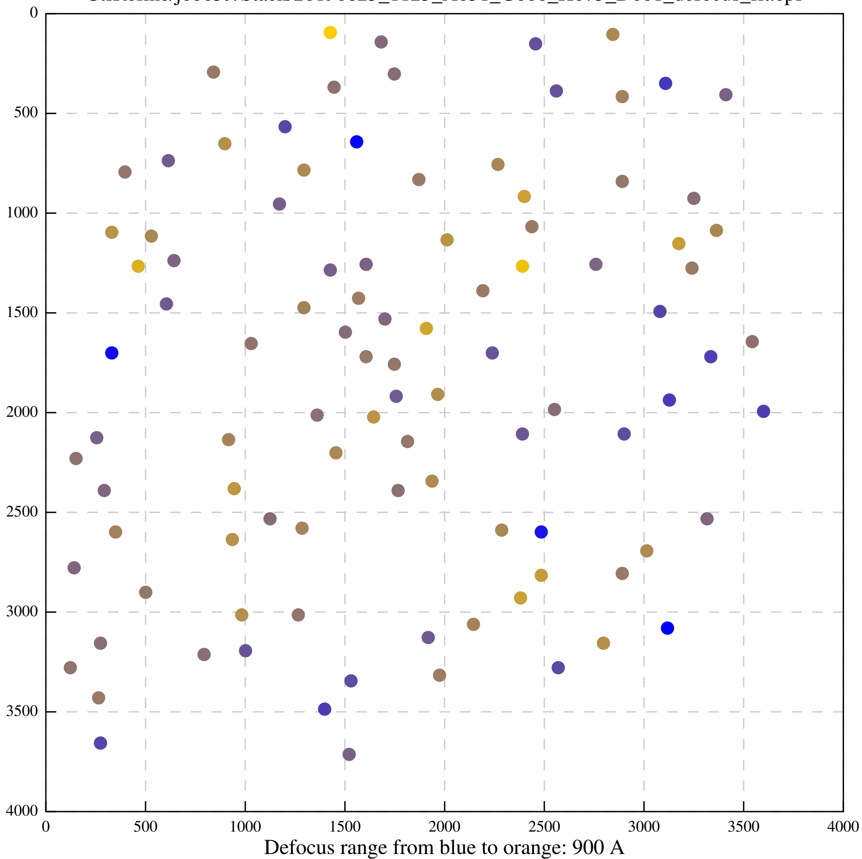
CtfRefine/job059/Stack/20190625_1125_A031_G000_H075_D001_defocus_fit.eps
